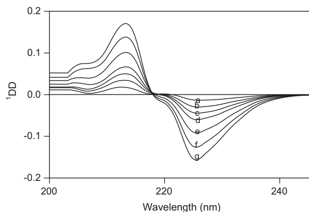
Figure 2 First derivative of the ratio method of a, 2; b, 4; c, 6; d, 8; e, 12; f, 16; g, 20 µg/ml solution of ibuprofen when 20 µg/ml solution of paracetamol used as divisor.
